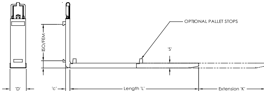
Reachforks Extended
